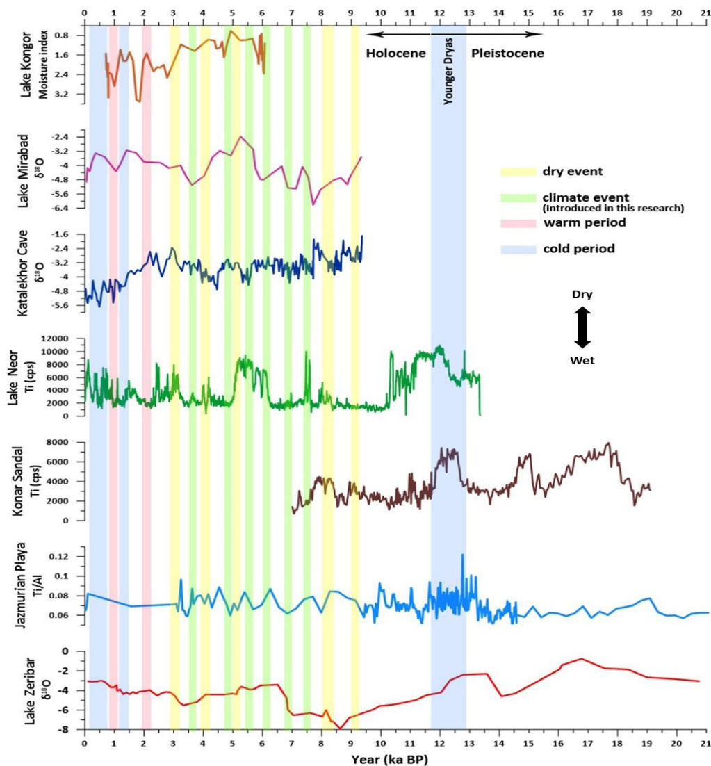
Figure 2. Paleoclimate research in Iran.
